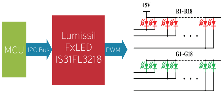
Fig - 8 Block Diagram
