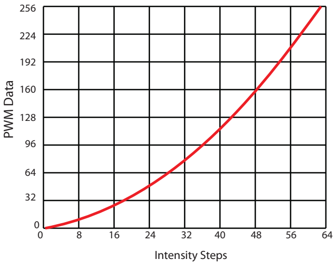
Fig 2 - Gamma Correction (64 steps)
