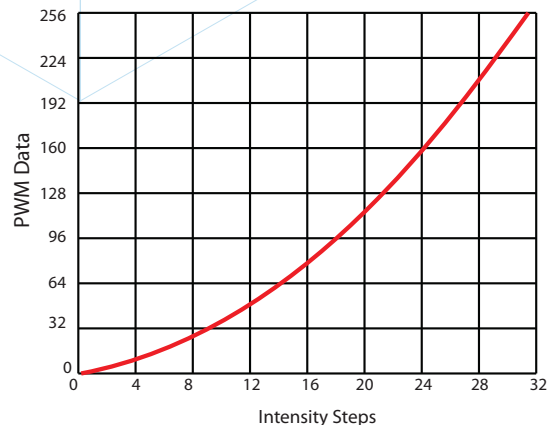
Fig 1 - Gamma Correction (32 steps)
